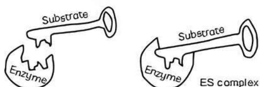
Induced fit model
