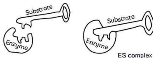
Lock and Key model
