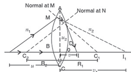
Refraction through a double convex lens
