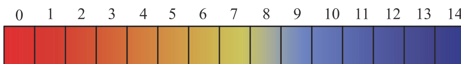
Fig. 8.7: Colour chart/guide of universal indicator/pH paper.
