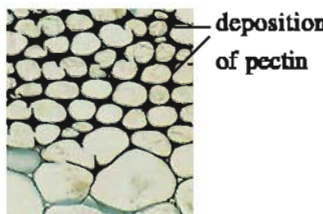
Collenchyma
