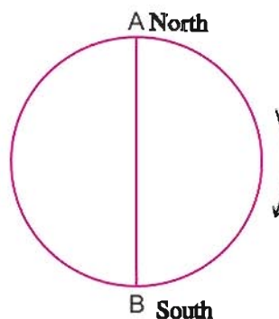
Figure 1.2 Circular path
