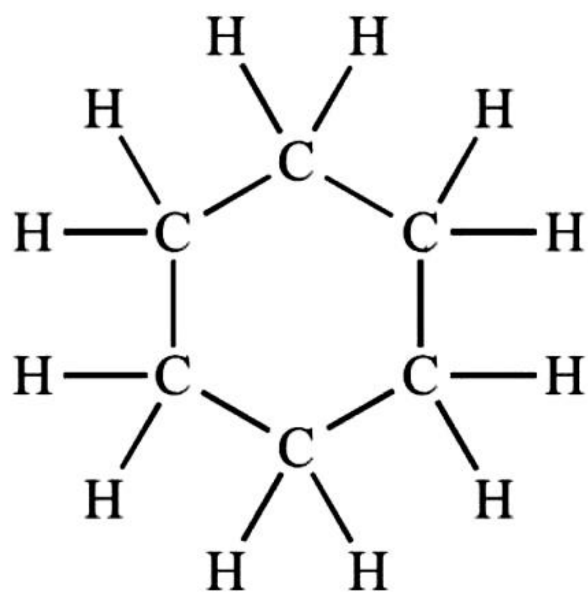
STRUCTURAL FORMULA OF CYCLOHEXANE &amp; ELECTRON DOT STRUCTURE
