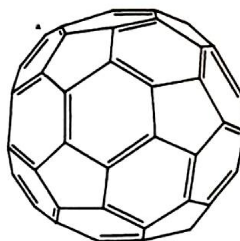
C 60 Buckyball
