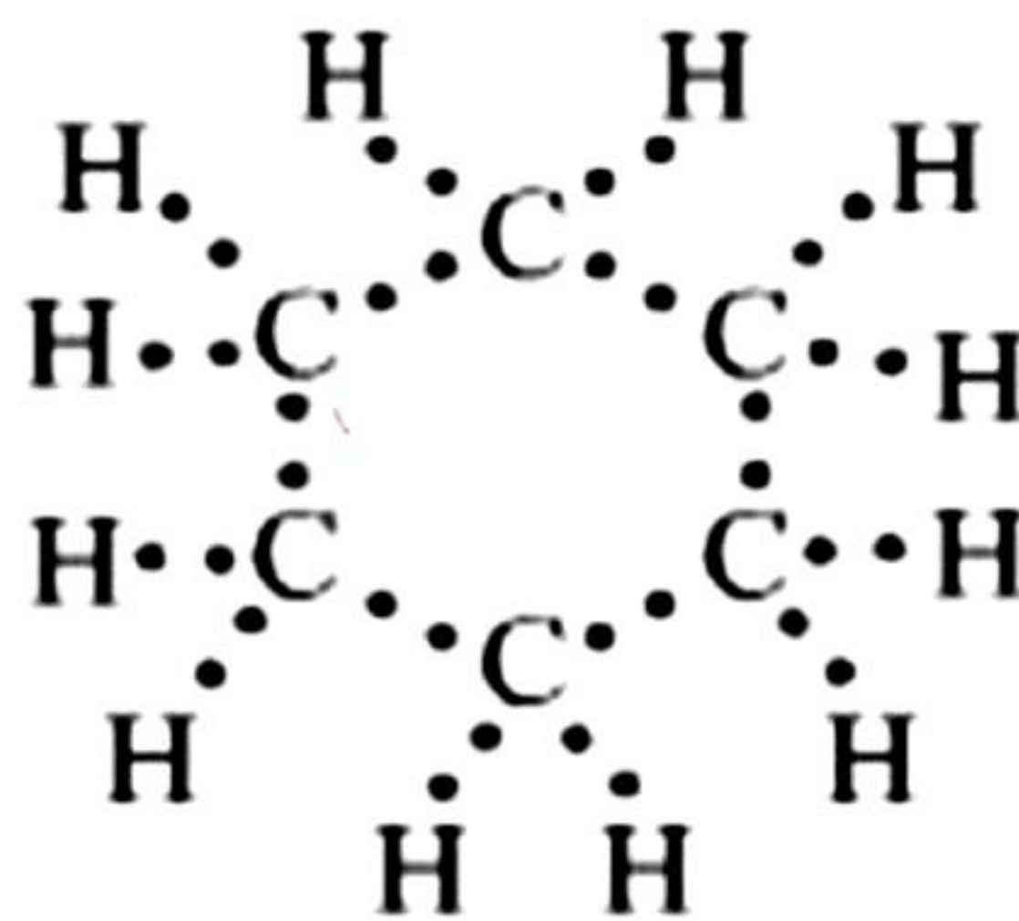
STRUCTURAL FORMULA OF CYCLOHEXANE &amp; ELECTRON DOT STRUCTURE
