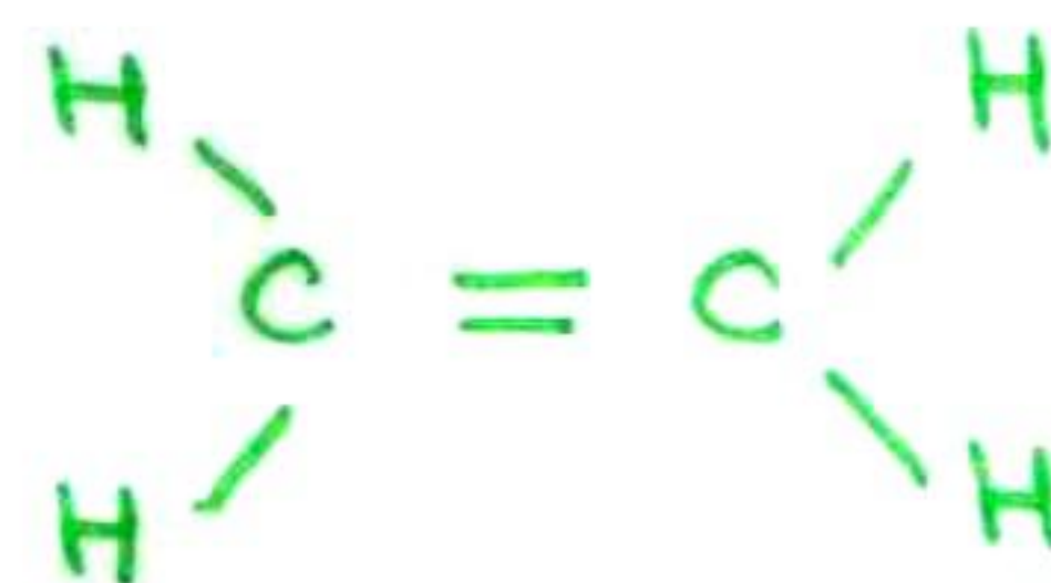
structural formula.
