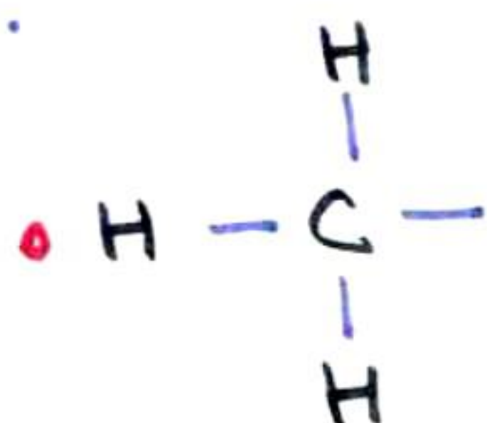
• Methyl group
