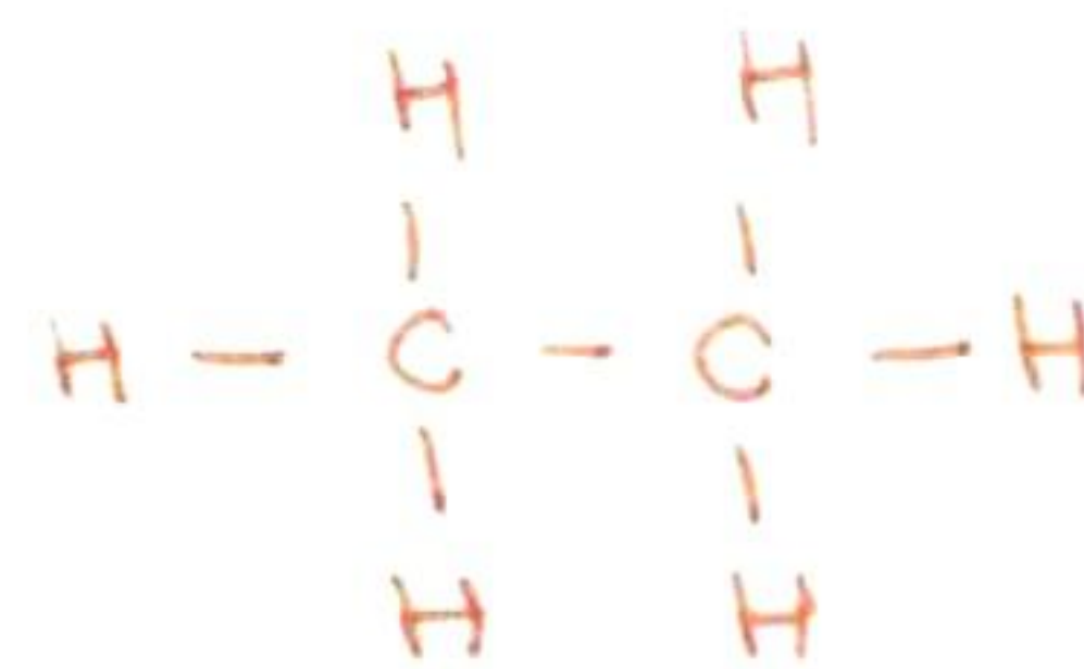
structural formula
