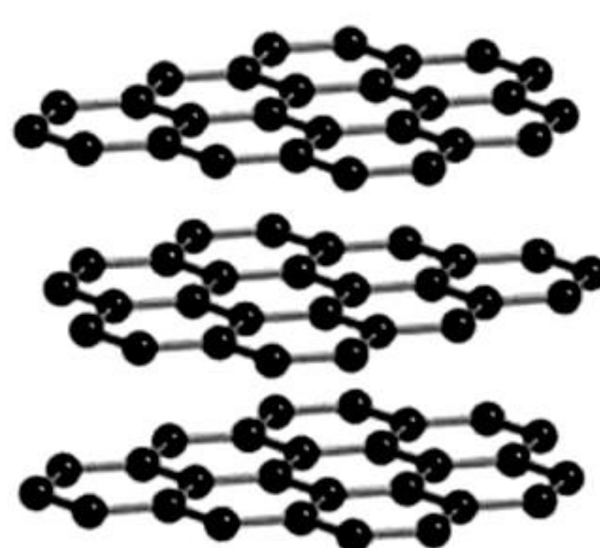
Graphite
