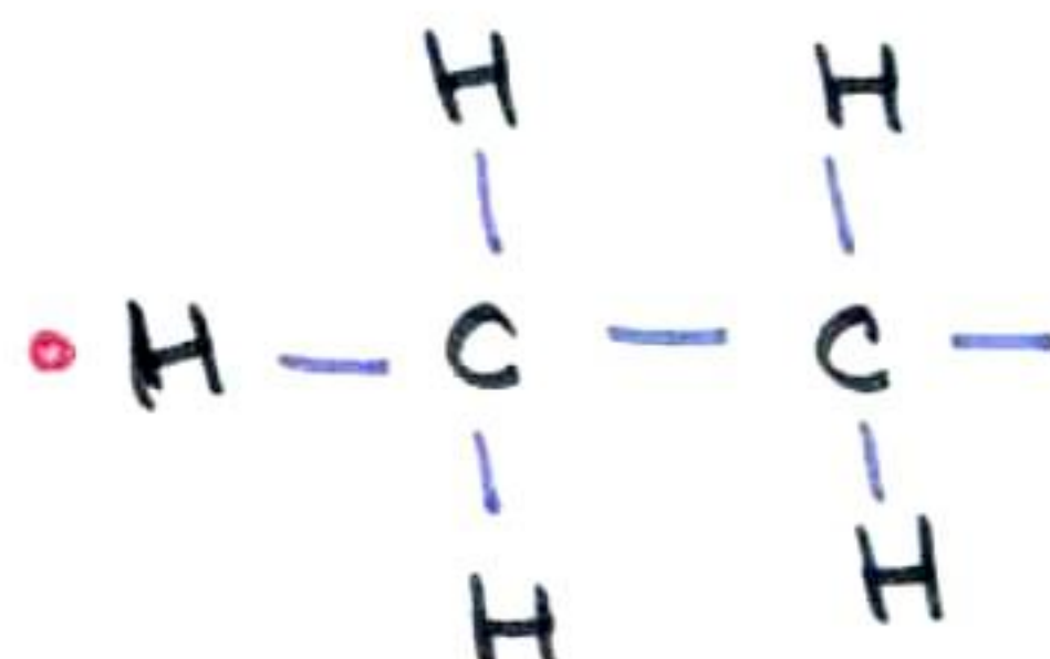
• Ethyl group
