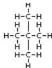
Neopentane
