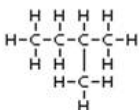
Isopentane
