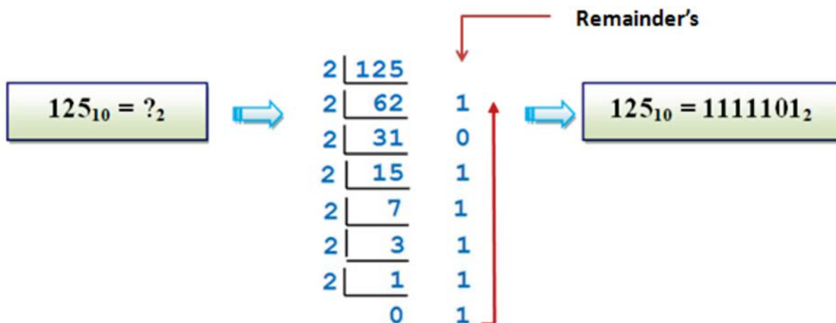
Figure 4.10 : Conversion Example
