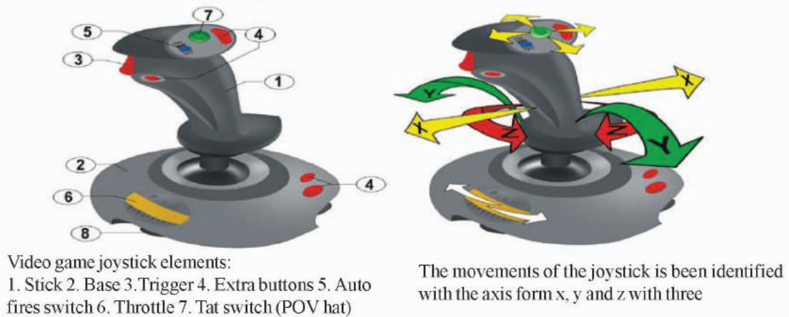
Figure 2.4 Joystick
