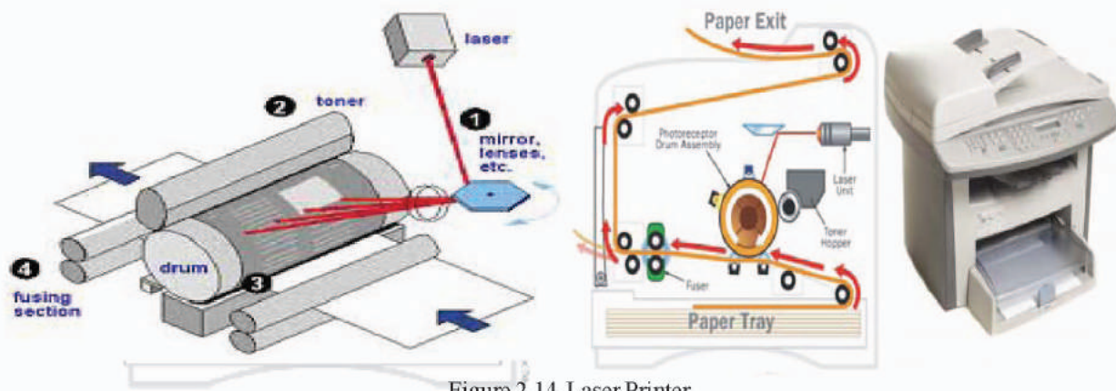
Figure 2.14 Laser Printer
