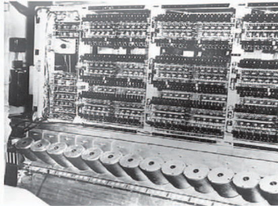
Figure1.16 EDVAC
