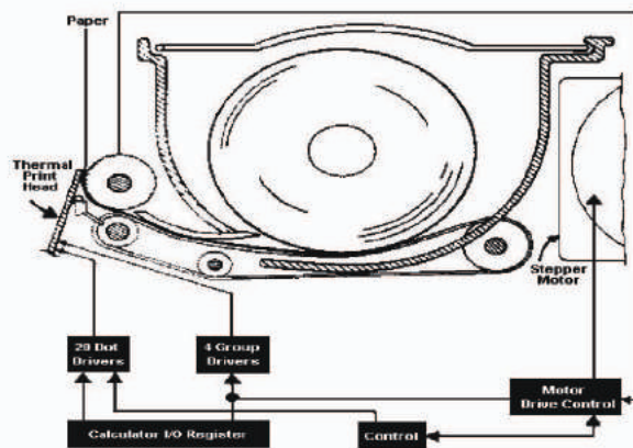
Figure 2.13 Thermal Printer
