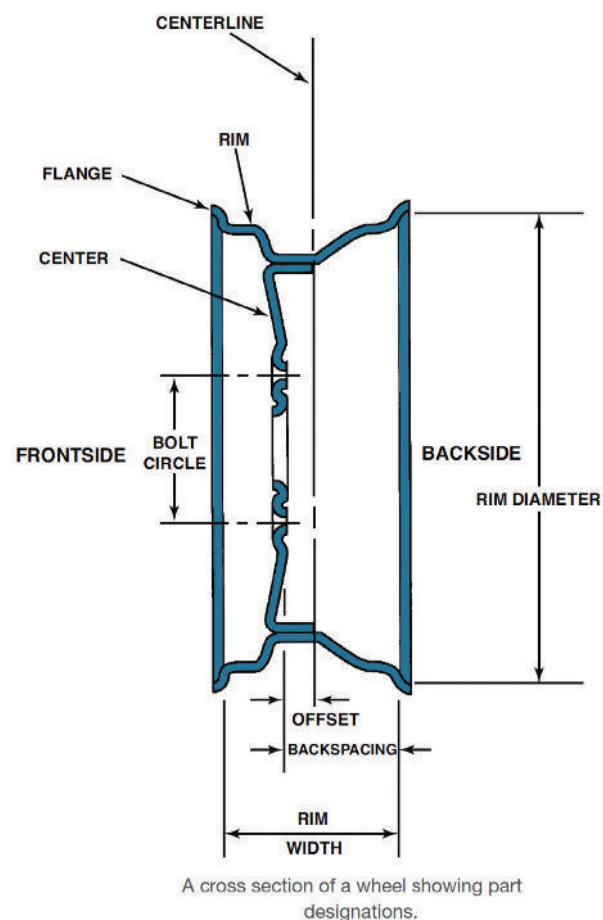
Figure 5.4 Wheel Dimensions
