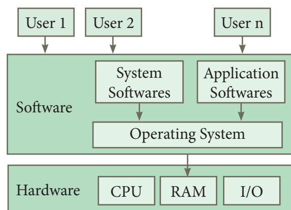
Figure 5.1. Overview of an Operating System
