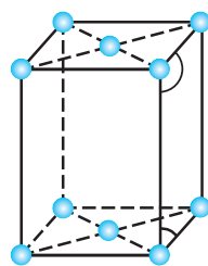
End-centred
