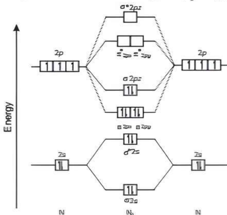
Molecular orbital diagram of \text{N}_2 molecule
