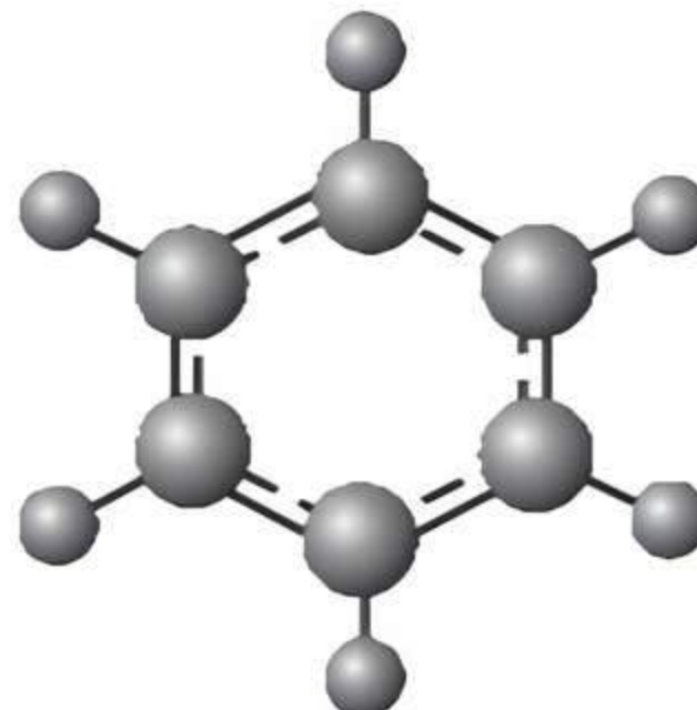
Benzene resonance Hybrid
