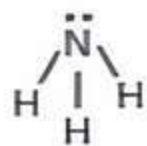
\text{NH}_3 molecule structure
