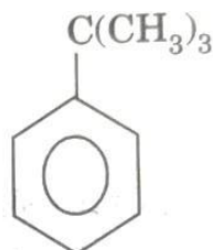
tert -butylbenzene
