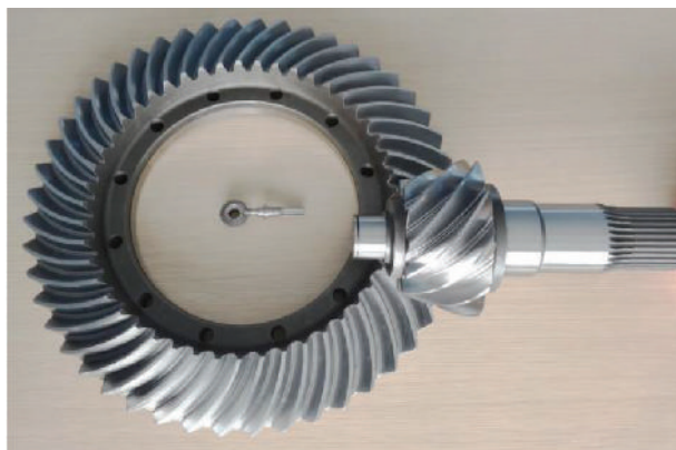
Figure 4.10.3 Hypoid bevel gear
