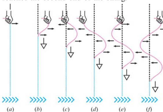
Figure 2.7 Transverse wave on a string
