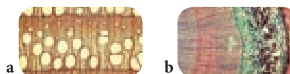
Figure 10.4: Structure of porous (a) and non-porous wood (b)
