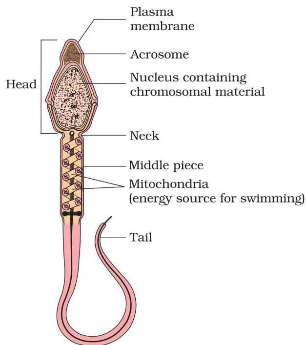
Figure 3.6 Structure of a sperm
