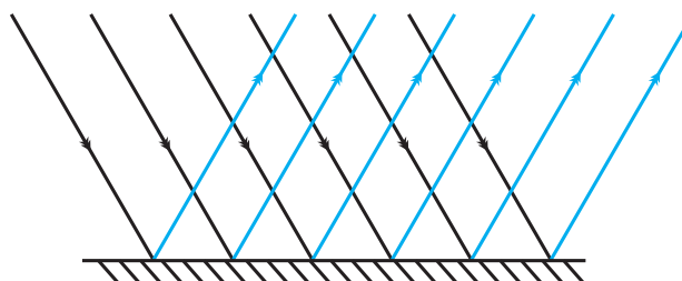
Fig. 16.8 : Regular reflection
