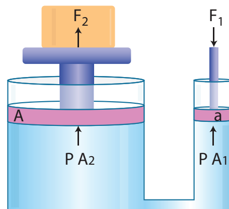
Figure 3.9 Hydraulic press
