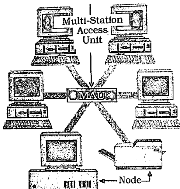
Fig.3. Star-wired ring topology
