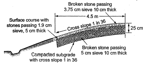
Figure-2.4: Typical cross-section of Macadam's construction
