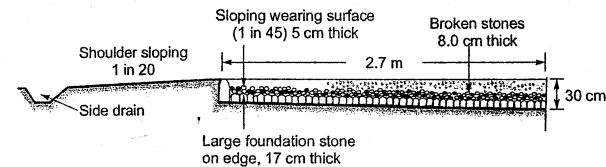
Figure-2.2: Typical cross-section of Tresaguet's construction
