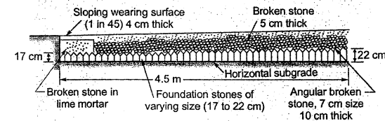
Figure-2.3 : Typical cross-section of Telford's construction
