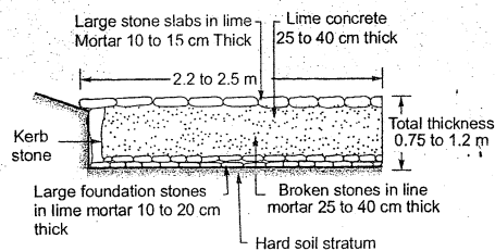
Figure-2.1 : Typical cross section of Roman Road
