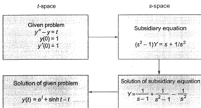
Laplace transform method
