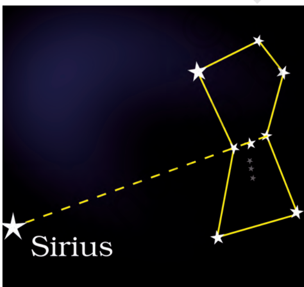
Fig. 17.15: Locating - Sirius
