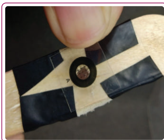
Fig. 2.4 , Grid fixed behind the lens of microscope
