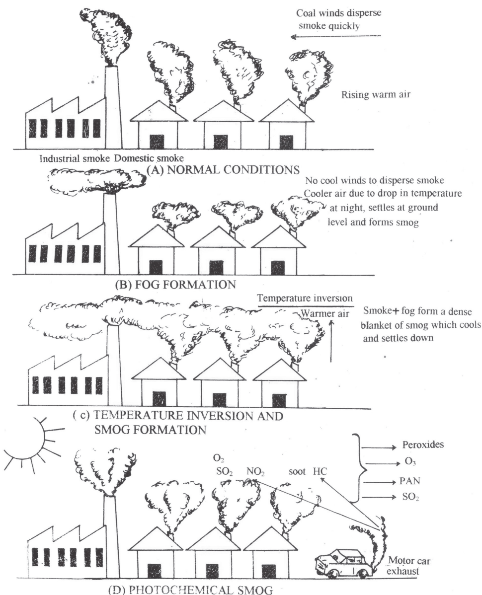
Fig. 30.13 Photochemical Smog
