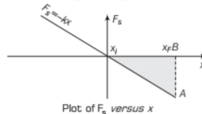
Plot of F_s versus x
