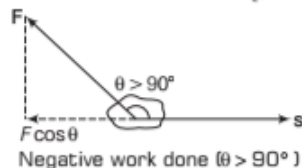
Negative work done ( \theta > 90^\circ )
