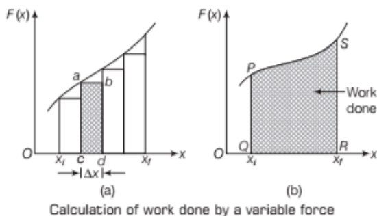
Calculation of work done by a variable force
