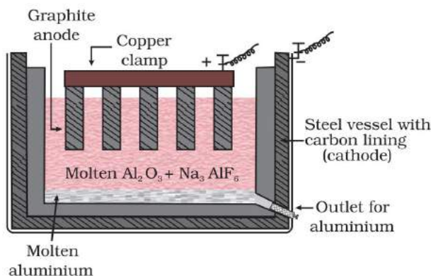
Fig. 6.6: Electrolytic cell for the extraction of aluminium
