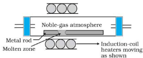
Fig. 6.7: Zone refining process
