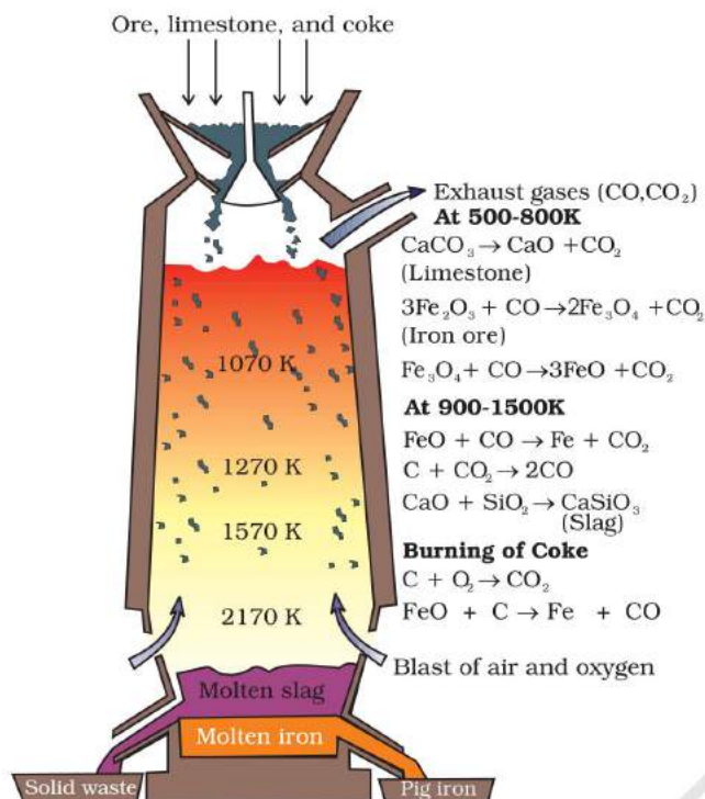
Fig. 6.5: Blast furnace
