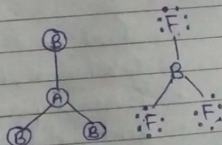
Trigonal planar
