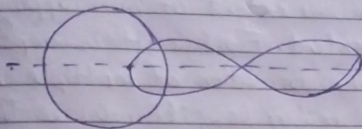
s-p overlap
