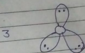
Trigonal planar
