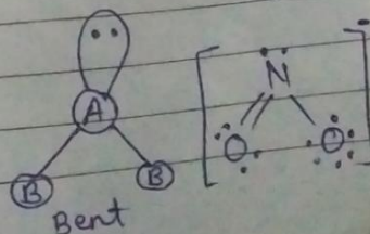
Trigonal planar
