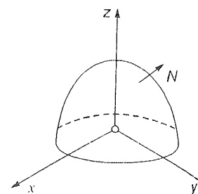
Surface S in Example 1
