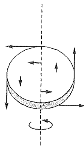
Velocity field of a rotating body
