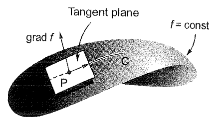
Gradient as surface normal vector
