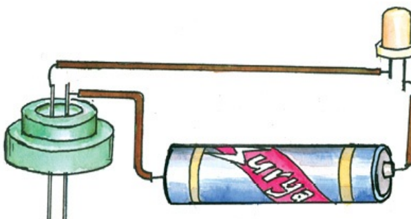
Fig. 2: Testing conductivity of liquids
