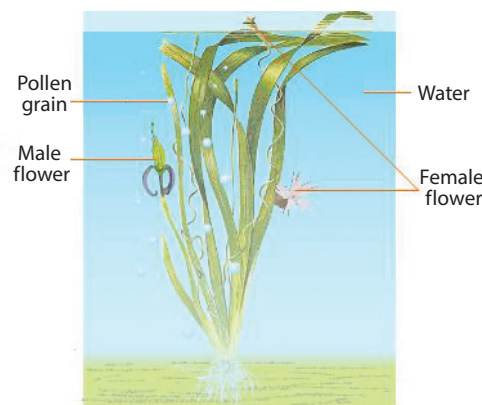
Figure 17.11 Hydrophily
