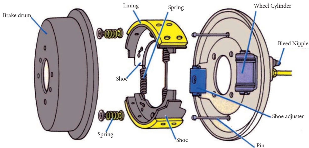
Figure 1.8.11 Braking system
