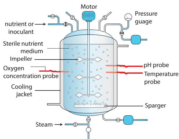
Figure 4.1: Bioreactor
