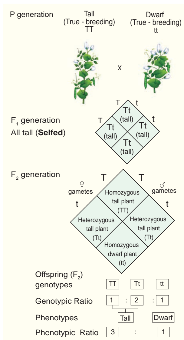
Figure 2.6: Monohybrid Cross
