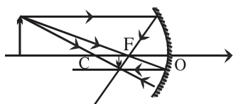
Fig 9.13 (c) Object far from centre of curvature
