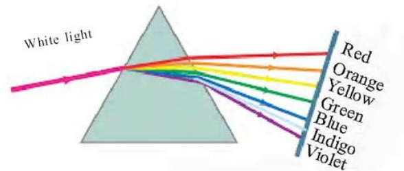
Fig. 9.22 Dispersion of white light
