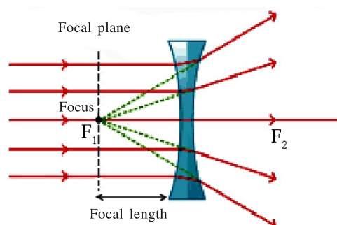
(b) Concave lens
