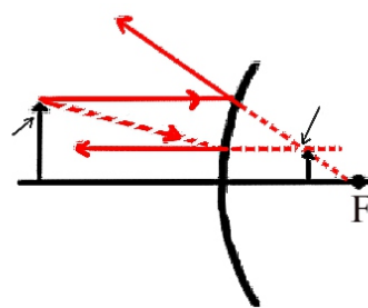
Fig 9.14 (c) object at certain distance
