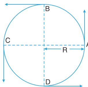
Fig. 9.31 Circular motion
