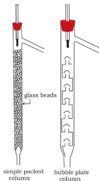
Fig.12.7 Different types of fractionating columns.
