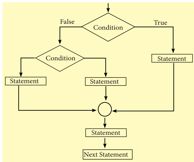
Flowchart 10.2 If nested inside else part
