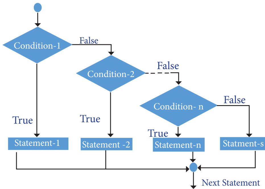
Flowchart 10.4 if-else ladder flow chart
