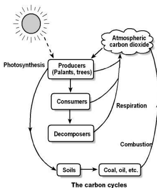
Fig. 9.3 : Carbon cycle
