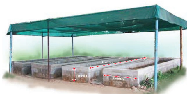
Figure 13.1 Vermiculture unit and Earthworms
