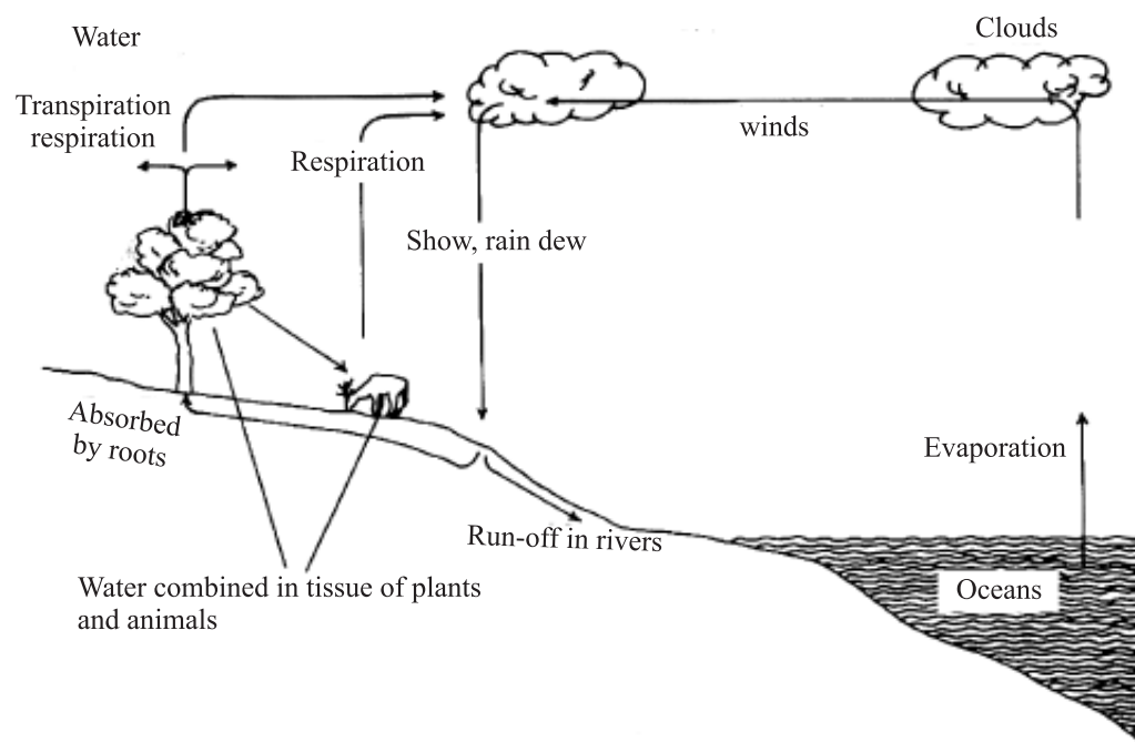
Fig. 26.1 Hydrological cycle
