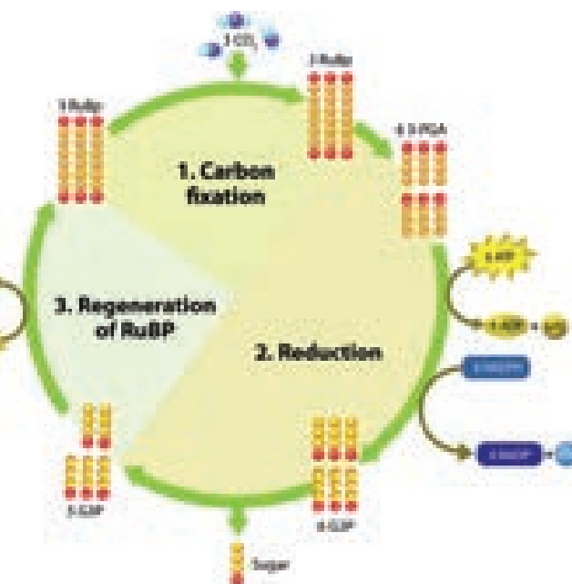
Figure 13.16: Phases of Calvin Cycle
