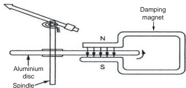
Fig. 6.5 Eddy current damping
