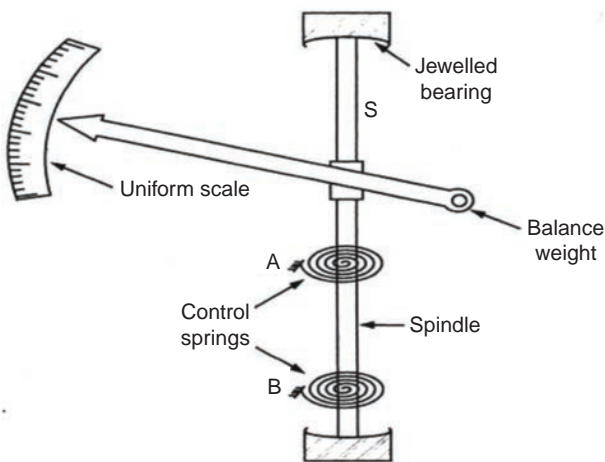
Fig. 6.1 Spring control
