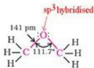
Methoxymethane (Ether)
