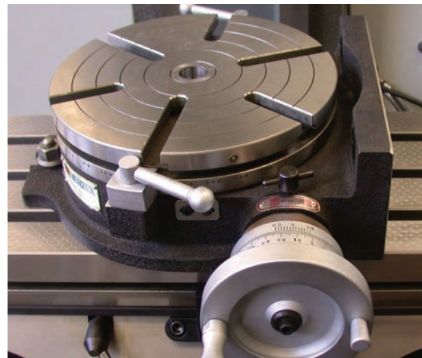
Rotary Table Milling Attachment
