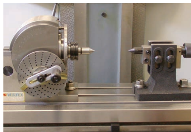
Indexing head attachment
