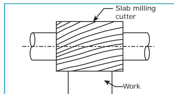
Horizontal milling
