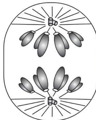
Anaphase
