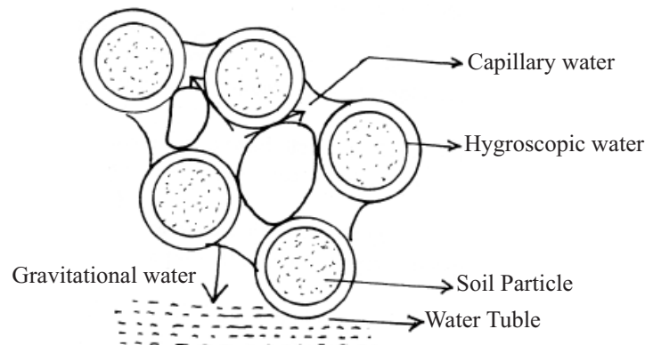
Fig. 8.6 Types of soil water.
