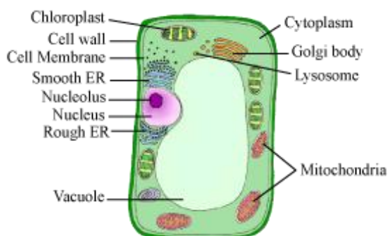
Plant cell
